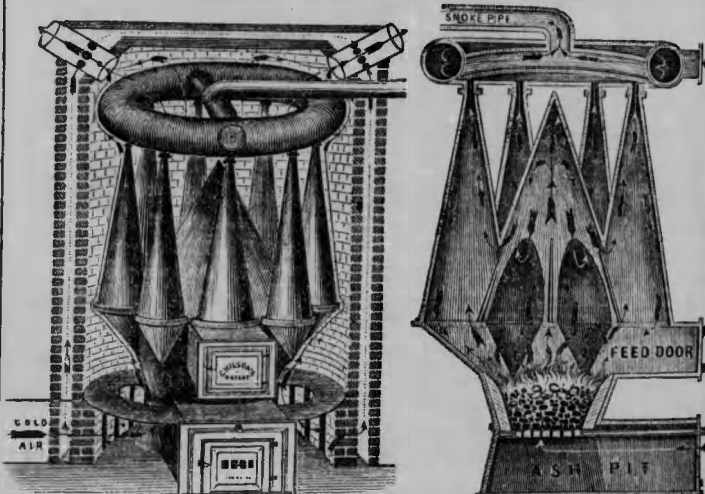
Elevation of Furnace and Section of Brick Work. Vertical Section, through Fire Pot, Cones and Annular Chamber, showing the Action of Heat on the Cones
