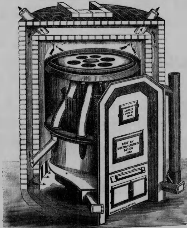
MAGEE'S NEW PATENT BRICK FURNACE.
