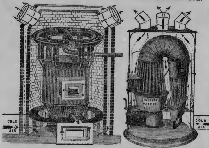
PORTABLE FURNACE.
